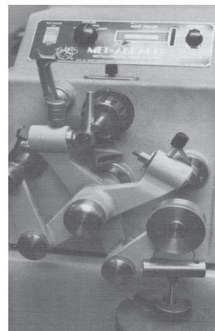
Taber Met-Abrader crossed cylinder wear test.
