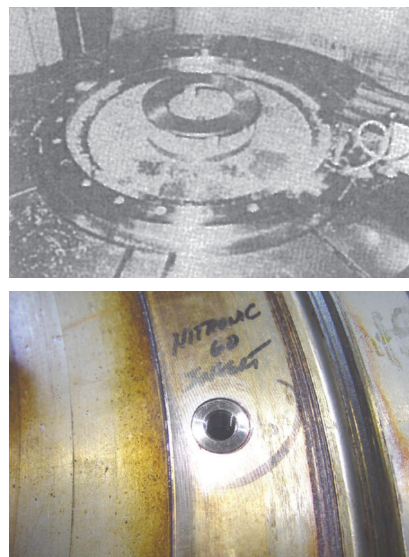
Wear Rings
